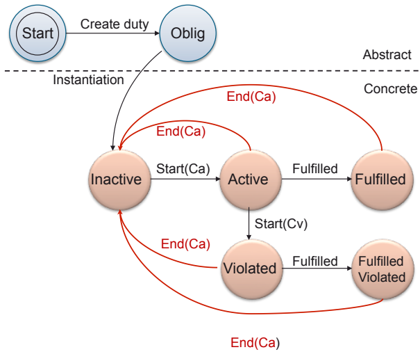
Fig. 2. State Transitions of Individual Obligations
