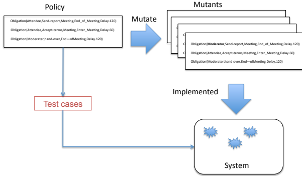
Fig. 4. Obligation mutation process
